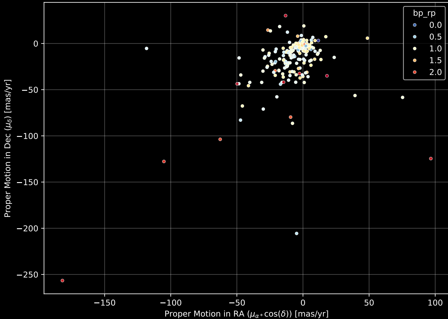
APOGEE DR17 Field: [182+33_MGA] Proper Motion Diagram (n= 206)
