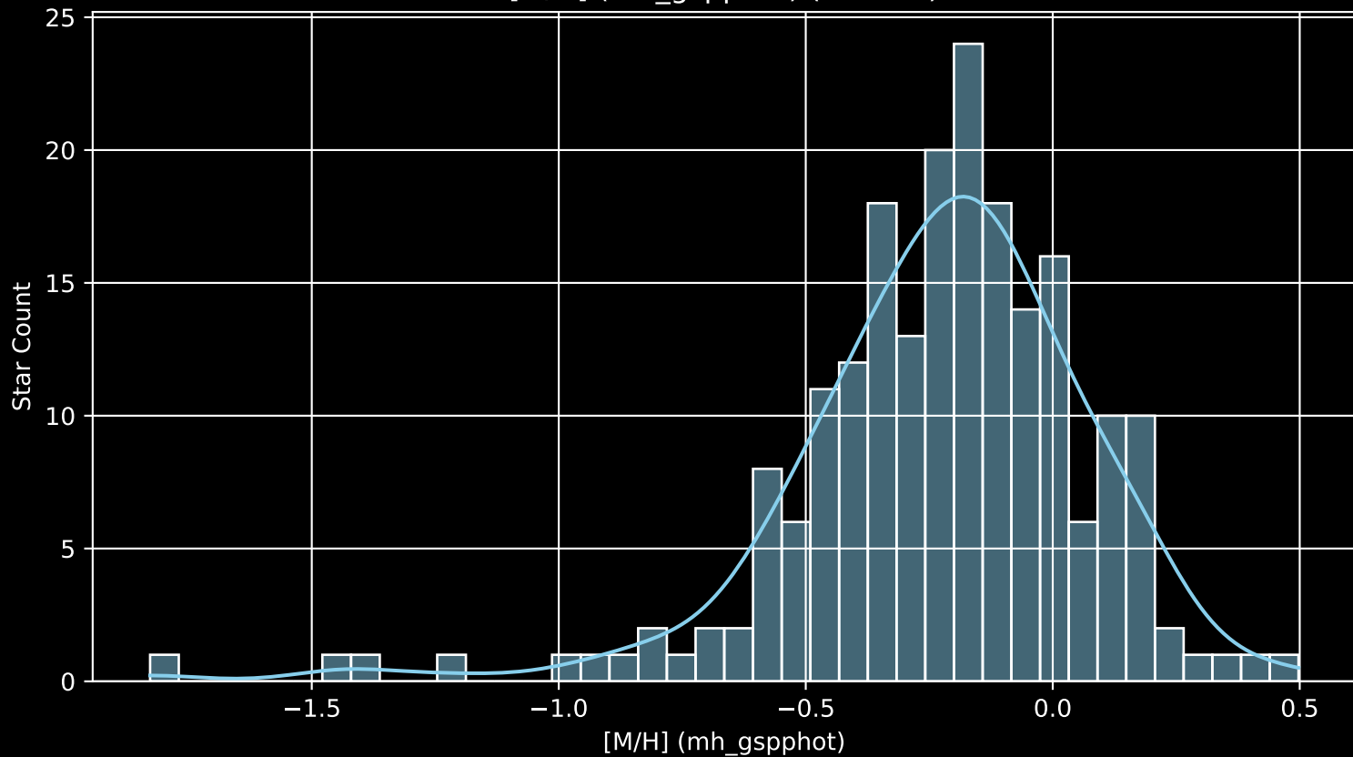
APOGEE DR17 Field: [182+33_MGA [M/H] (mh_gspphot) (n= 206)
