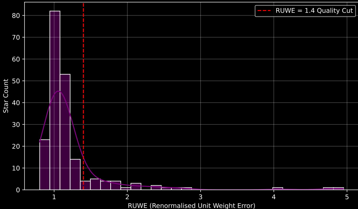
GAPOGEE DR17 Field [182+33_MGA] RUWE Distribution (n= 201)
