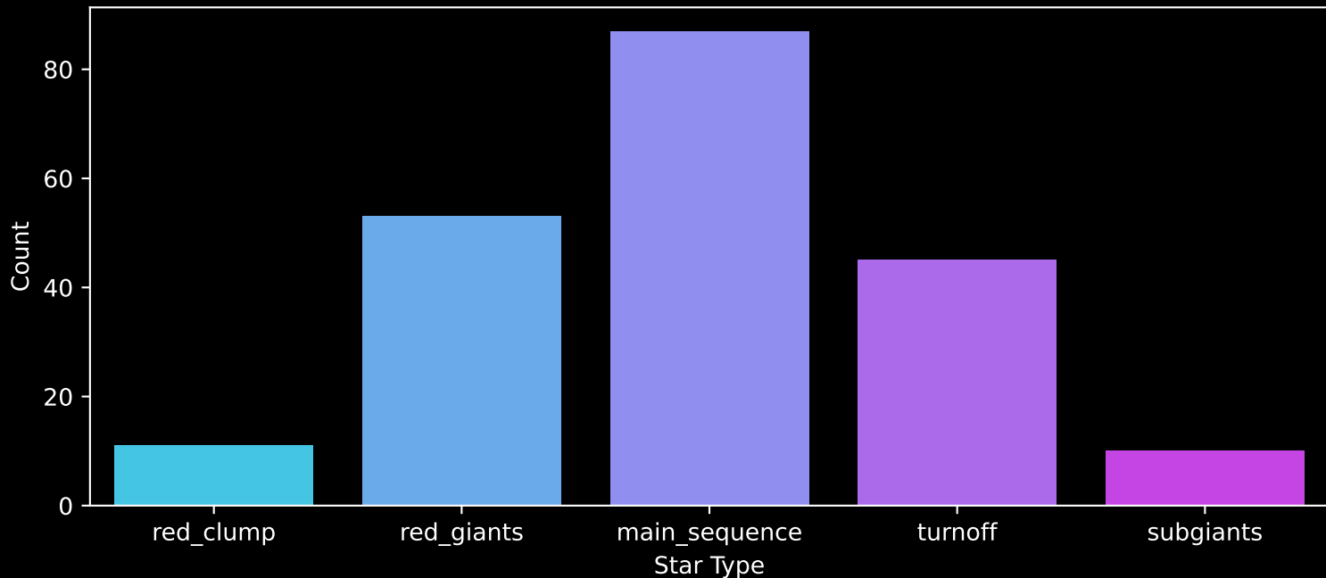
APOGEE DR17 Field: [182+33_MGA] Count plot of Star Type
