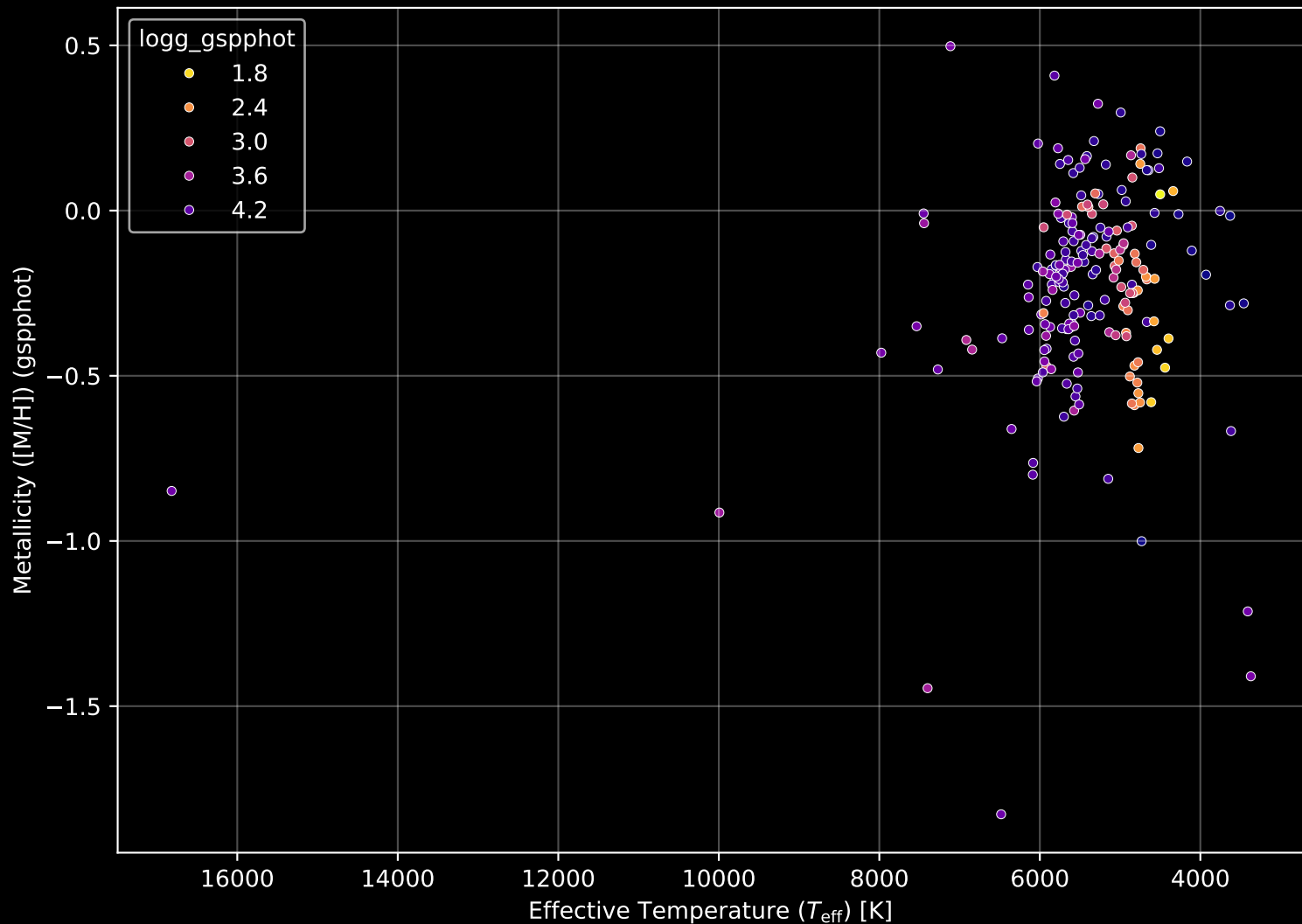
APOGEE DR17 Field: [182+33_MGA] Stellar Population Parameters (n= 206)
