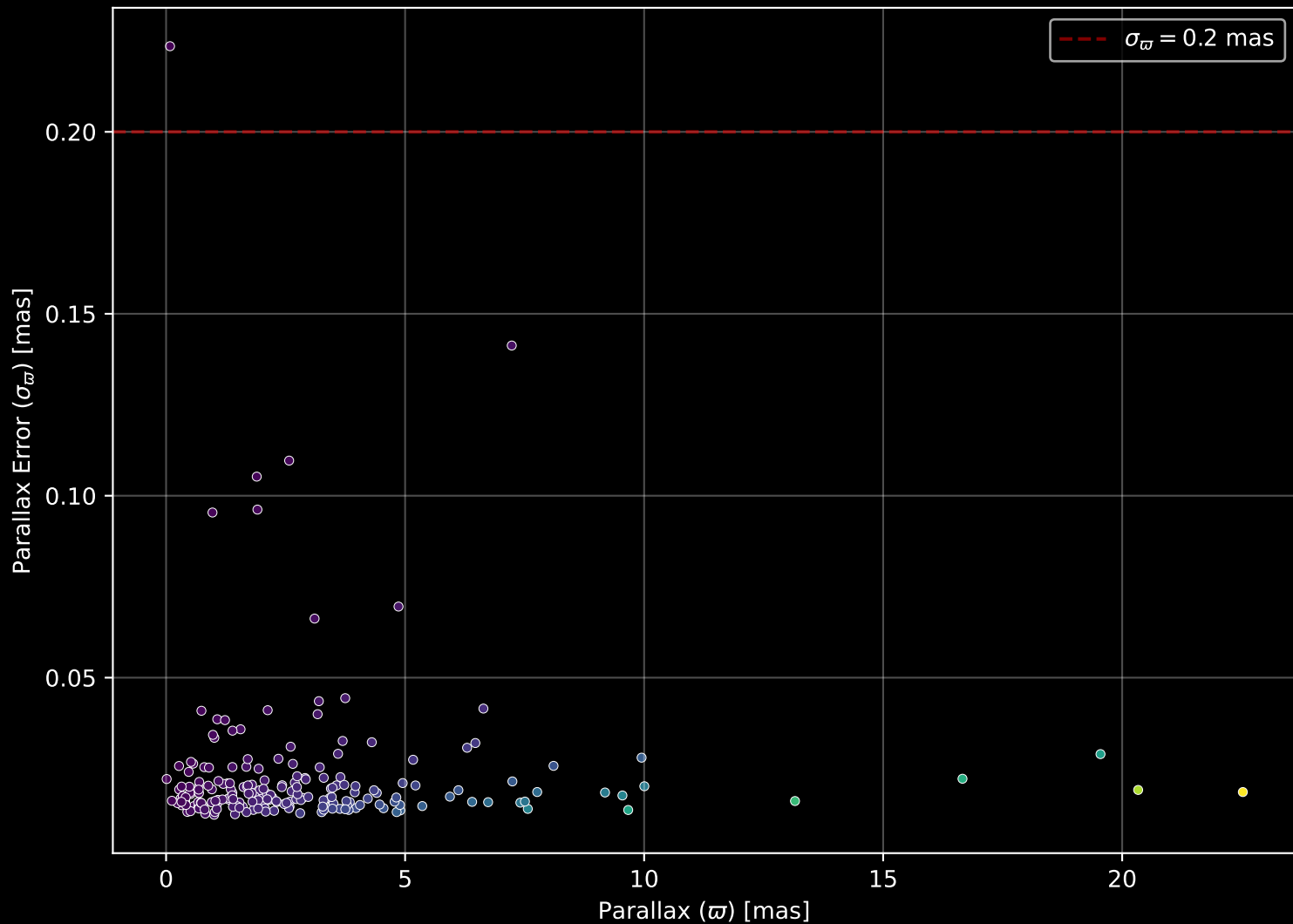
APOGEE DR17 Field: [182+33_MGA] Parallax Quality (n= 206)
