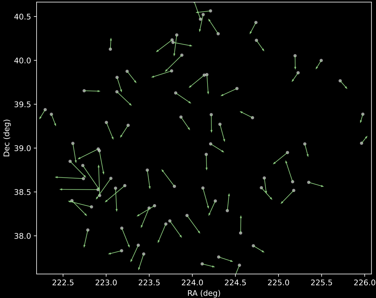
APOGEE DR17 Cluster 5 Proper Motion Vectors (n=76)
